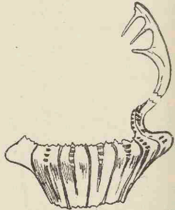
FIG. 550. Williamsonia gigas . Side-view of an incomplete staminate disc showing the basal cup torn at the lower end and part of one of the free microsporophylls. (Diagrammatic drawing, after Thomas; nat. size.)
