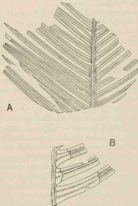
FIG. 617. Pseudocycas insignis . From the Lias of Hör. A, \frac{1}{2} nat. size; B, ca. \times 2 . (After Nathorst.)
