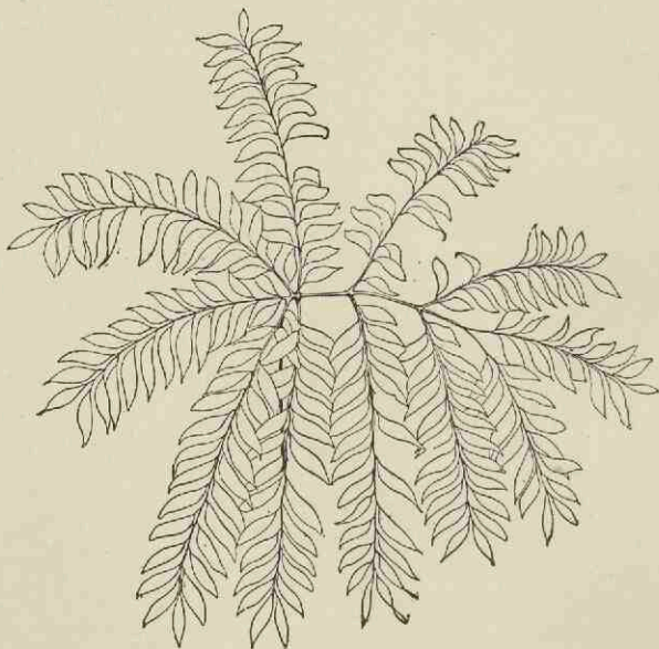
FIG. 391. Bowenia spectabilis , frond. (From the Encyclopaedia Britannica .)
