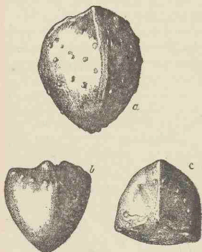
FIG. 584. Carpolithus conicus . The type-specimens in the Manchester Museum; nat. size. (a, No. 361; b, c, No. 360.)
