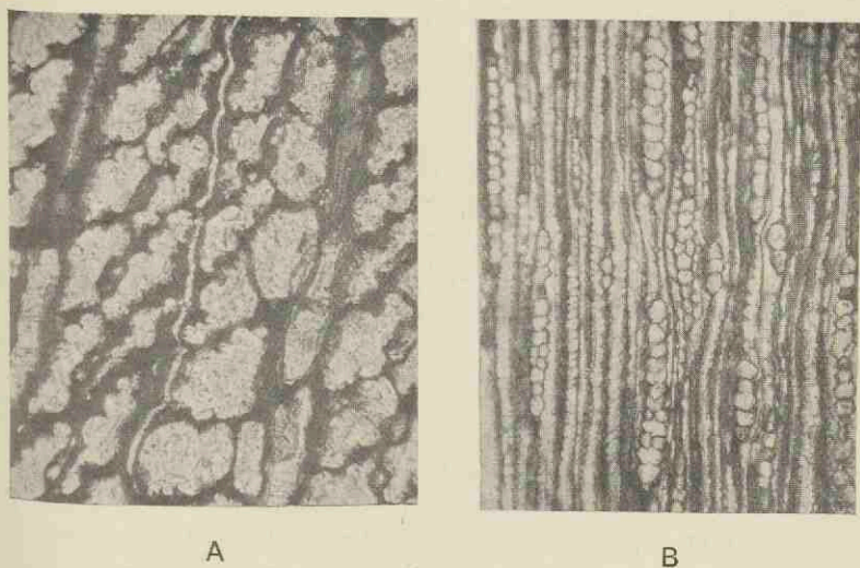
FIG. 474. Dadoxylon materiaram . Transverse (A) and tangential (B) sections of the secondary xylem. (Kidston Coll. 222, 224.)
