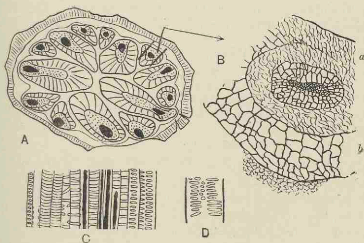
FIG. 461. Völkelia refracta . A. Transverse section of a specimen in the Breslau Museum. B. Portion of a stele; a, the crushed xylem on the outer side; b, the inner side. C. Longitudinal section showing the median protoxylem. D. Tracheid from the secondary xylem. (After Solms-Laubach.)
