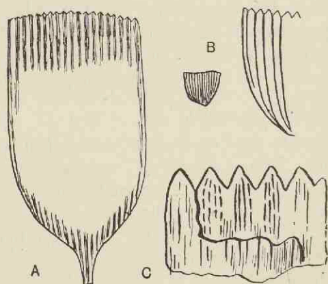
FIG. 428. A, C. Whittleseya elegans . A, single leaflet, from Pennsylvania. (After Lesquereux; \frac{2}{3} nat. size.) C, diagrammatic sketch of part of a leaflet showing the teeth, the striated texture of the carbonised layer, and the vein-like markings on a lower surface. (After Thomas; enlarged.)
