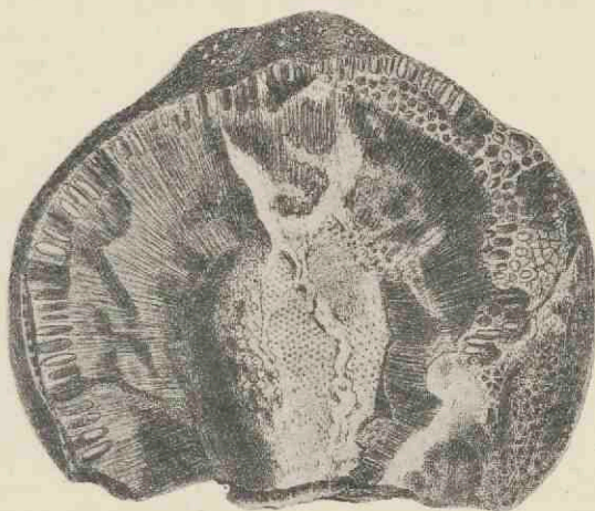
FIG. 560. Williamsonia Bucklandi . (After Buckland; \frac{1}{2} nat. size.)
