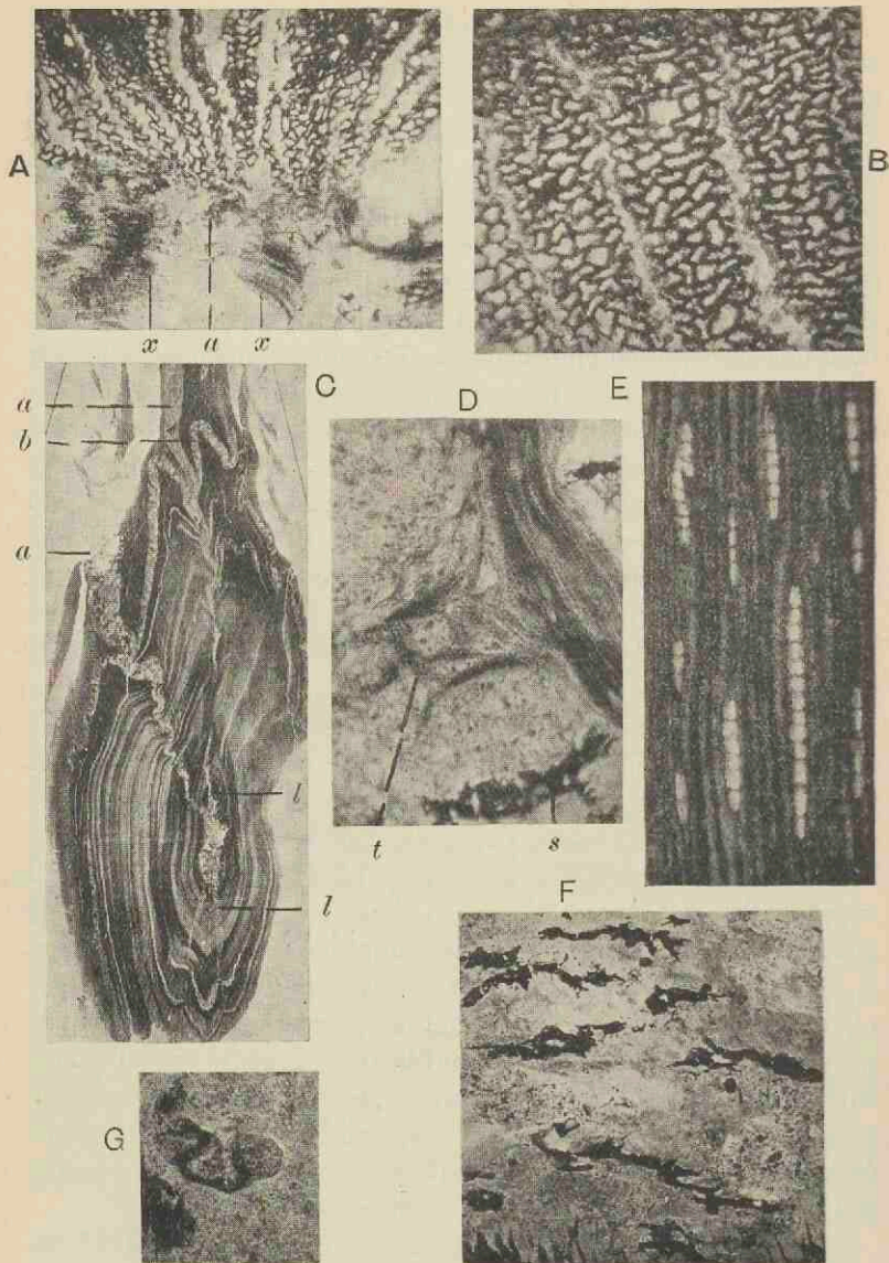
FIG. 491. A—F, Antarcticorylon Priestleyi . A, B, transverse sections of the xylem; a , small tracheids simulating protoxylem; x , xylem at the edge of the pith. C, transverse section showing leaf-traces, l , a , b . D, leaf-trace with short tracheids, t , in the pith; s , sclerous cells. E, tangential section. F, pith in longitudinal section. G, Pityosporites antarcticus ; see Vol. IV. (All the sections are in the British Museum.)
