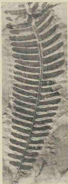
FIG. 616. Pterophyllum ( Anomozamites ) Lyellianum . (Geological Survey Museum, 6396; nat. size.)
