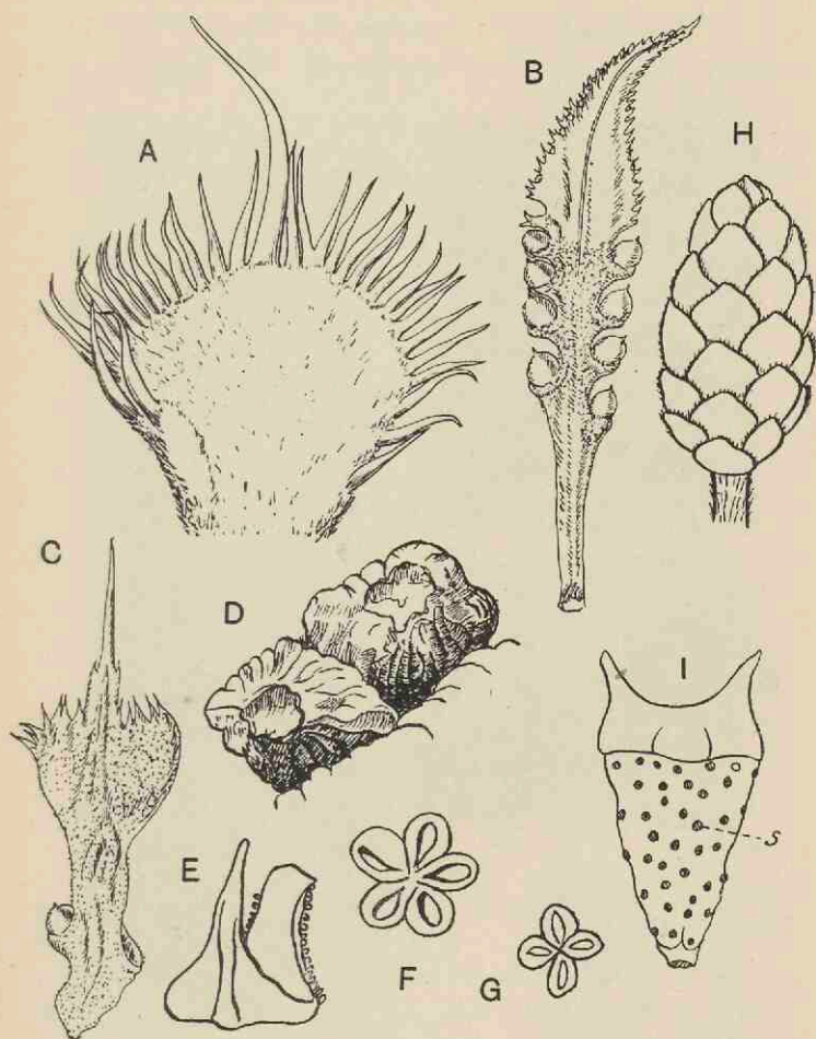
FIG. 392. A. Cycas pectinata , apex of megasporophyll. ( \frac{2}{3} nat. size.) B, C. Cycas Ruminiana , megasporophyll. ( \frac{2}{3} nat. size.) D. Encephalartos Allensteinii . Distal end of megasporophylls. (From the Gardeners' Chronicle .) E, F. Cycas angulata , microsporophyll and sorus. G, I. Ceratozamia mexicana , I, microsporophyll with scars of sori ( s ); G, sorus. (After Thibout.) H. Stangeria paradoxa , megastrobilus.
