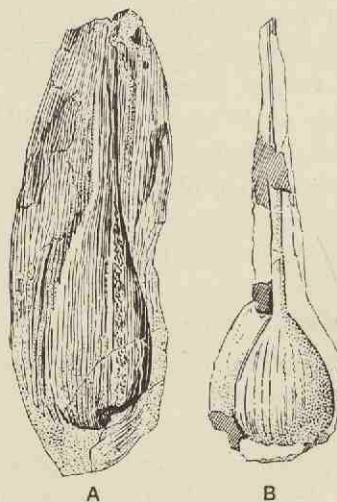
FIG. 425. Trigonocarpus Parkinsoni . A. Impression showing the nucule and sarcotesta. (= Carpolithes alata Lind. and Hutt.) B. Specimen with long micropyle. (A, nat. size; from the Lower Coal Measures of Kilmarnock; B, nat. size; Middle C. M. of Yorkshire. Kidston Coll., 1579 and 1062.)
