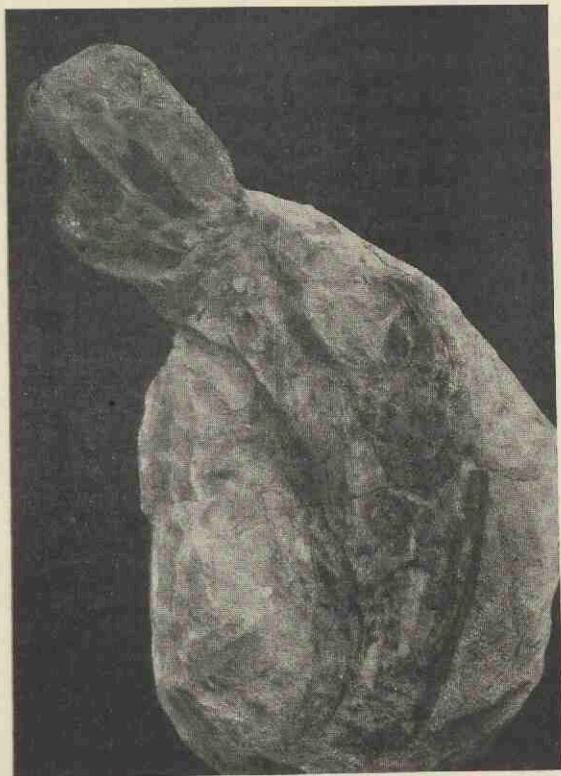
FIG. 542. Williamsonia gigas . Flowering shoot and flower-bud. (Yates Collection, Paris.)
