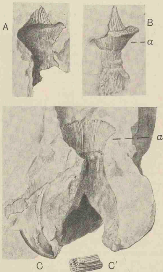
FIG. 546. Williamsonia gigas . A, apical portion of flower. B, cast of A; a, persistent interseminal scales. C, flower in longitudinal section. C', interseminal scales from the base. (Williamson Collection, Botany School, Cambridge.)
