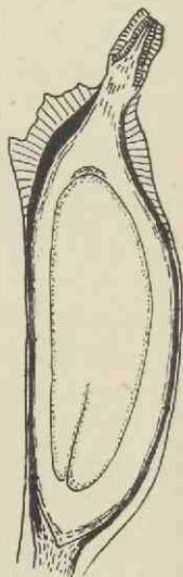
FIG. 516. Cycadeoidea Dartoni . Longitudinal section of seed with embryo. (After Wieland; \times 19 .)
