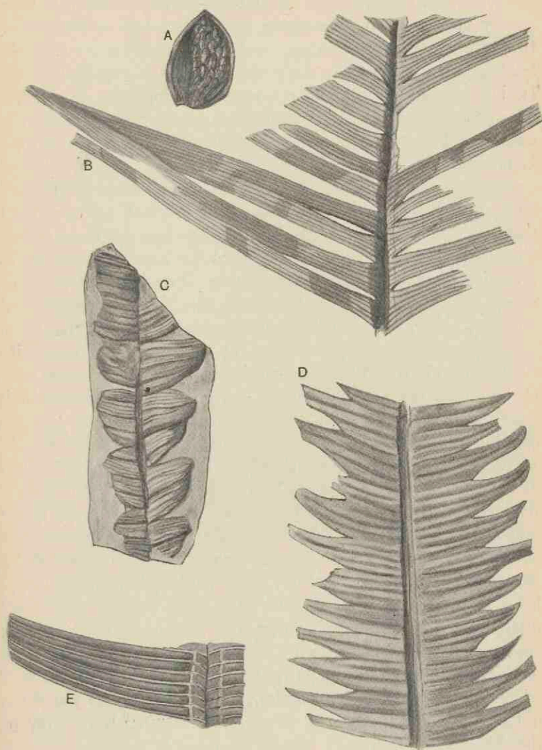
FIG. 619. A, seed ( Nilssonia ?); B, Nilssonia pterophylloides ; C, D, Nilssonia brevis ; E, N. polymorpha . (A—D \frac{5}{8} nat. size; E, slightly enlarged; after Nathorst.)
