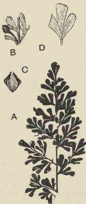
FIG. 445. Wardia fertilis (White). A, sterile portion of frond; B, D, enlarged pinnules; C, seed. (After White. A, ca, nat. size; B—D, \times 2 .)
