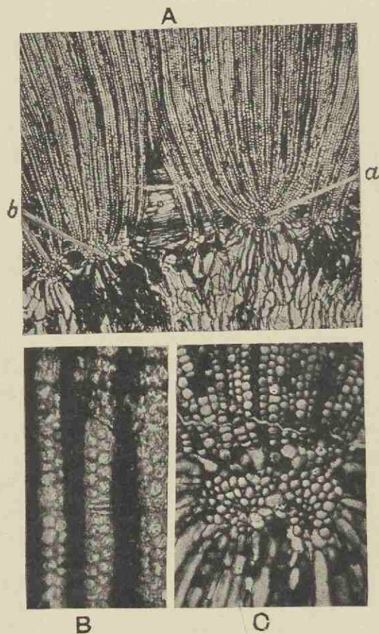
FIG. 489. Callixylon Trifilievi . A, C, the inner margin of the secondary xylem showing strands of primary xylem, a, b, and C. B, tracheids of the secondary xylem. (A, C, from photographs supplied by Prof. Zalessky; B, Cambridge Botany School.)
