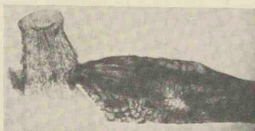
FIG. 554. Williamsonia Leckenbyi . Micropyle and interseminal scale. (After Nathorst.)
