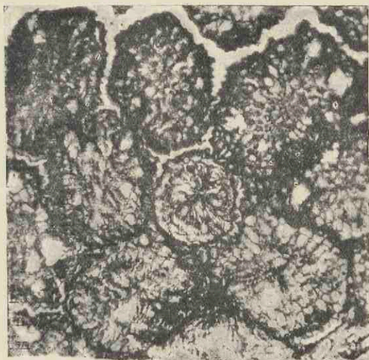
FIG. 564. Williamsonia scotica . Transverse section near the distal end of a micropylar tube and the surrounding polygonal interseminal scales. (ca. \times 100 .)
