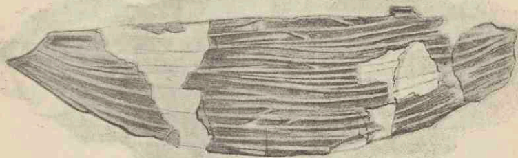
FIG. 624. Ctenis sp. Single pinna. (Manchester Museum, No. 53.)
