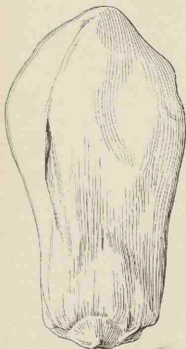
FIG. 582. Cycadolepis ( Eury-Cycadolepis ) sp. From the Wealden beds of Sussex. (Brit. Mus. No. V. 2799.)
