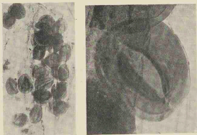
FIG. 429. Microspores of Whittleseya elegans . A, a group of spores; B, a single spore. (Preparations made from an American specimen, No. 2314, in Dr Kidston's Collection.)
