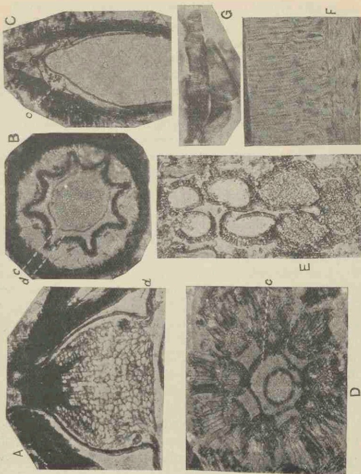
FIG. 493. A, Lagenostoma ovoides , longitudinal section of the lagenostome. B, Lagenostoma Lomaxi , transverse section of the lagenostome and canopy; c , pollen-chamber; d , space between the nucellus and integument. (A, after Miss Frankerd; B, from a section in the Manchester Museum, R. 1048.) C, Physostoma elegans , longitudinal section showing microspores in the pollen-chamber, c . (From a section in the University College Collection.) D, Physostoma elegans , transverse section of the apical region showing the tentacles, pollen-chamber, c , etc. E, Talamium Scotti , transverse section of sporangia (Manchester Coll. R. 1047). F, G, Stephanospermum alenioides . F, section of sclerotesta. G, tracheids from the nucellus. (University College Coll.)
