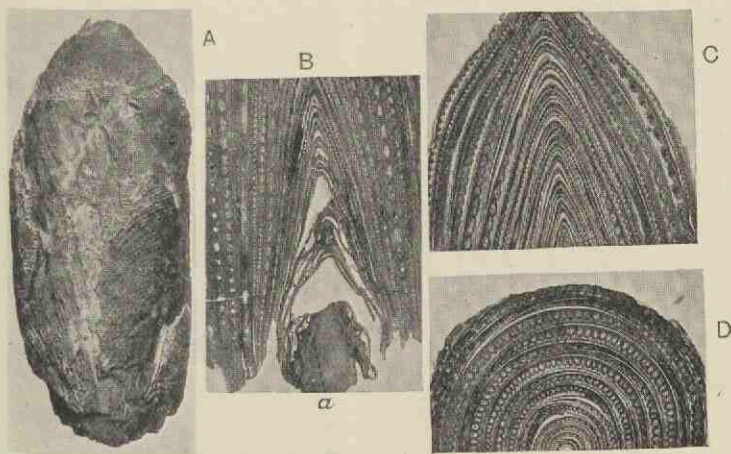
FIG. 430. Dolerophyllum Goepperti . Bud in surface-view, A; in longitudinal section, B, C; in transverse section, D. (British Museum; A, \frac{2}{3} nat. size.)
