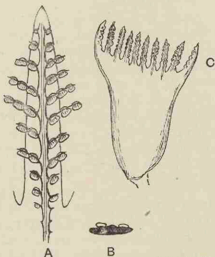
FIG. 565. A, Williamsonia spectabilis , microsporophyll; B, W. whitbiensis , section of sporophyll; C, W. mexicana . (A, B, after Nathorst; C, after Wieland.)
