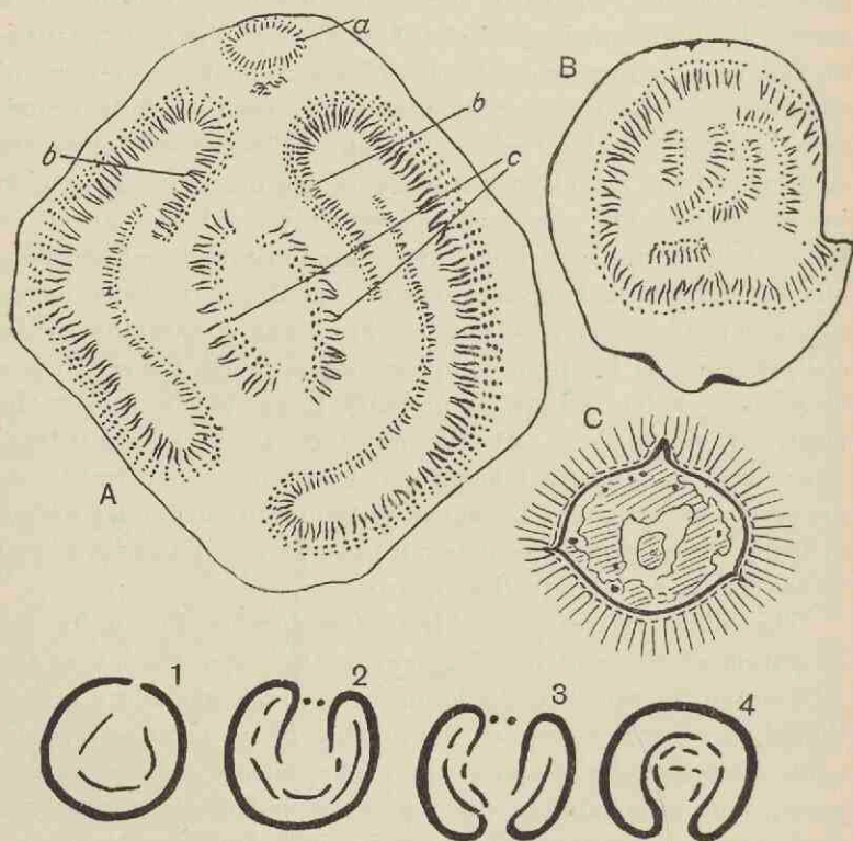
FIG. 453. A. Ptychoxylon Levyi ; transverse section of stem; a, stela of branch. (After Renault.) B. Cycadoxylon Fremyi ; transverse section of stem. (After Renault.) C. Cycadoxylon robustum ; centre of stem. 1—4, diagrams of sections of the stem of Ptychoxylon at different levels. (Simplified from Renault.)
