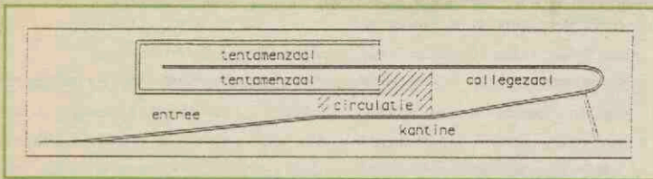
Dwarsdoorsnede Educatorium.
