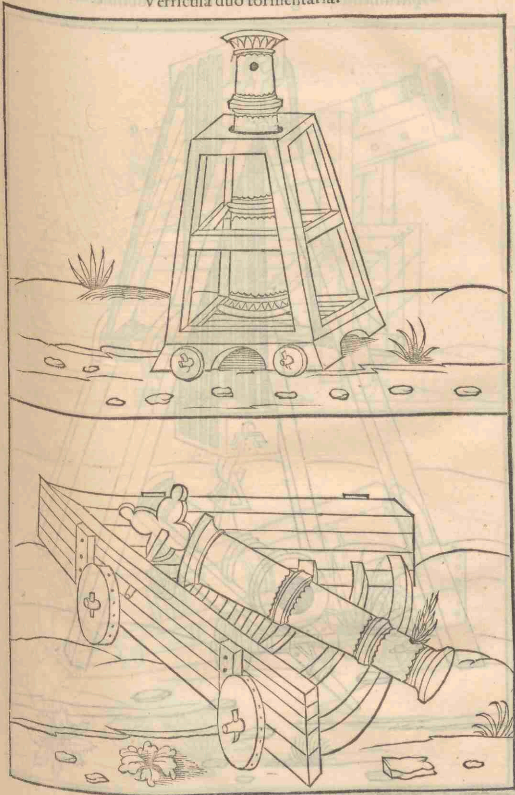
Verricula duo tormentaria.
